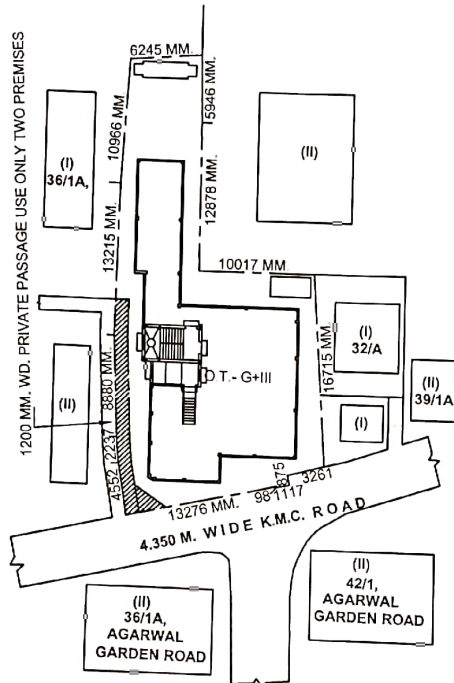
SITE PLAN SCALE = 1:600
